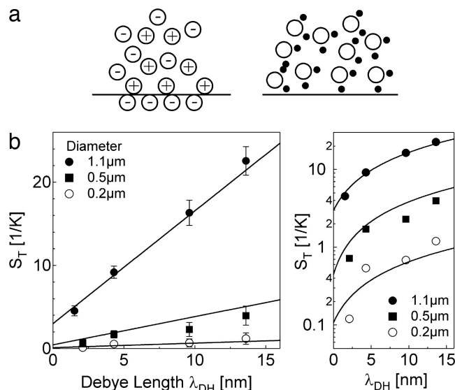
Fig. 2. Salt dependence. (a) Thermodiffusion in water is dominated by ionic shielding (Left) and water hydration (Right). (b) Soret coefficient \mathcal{S}_T versus Debye length for carboxyl-modified polystyrene beads of diameter 1.1, 0.5, and 0.2 \mu\text{m} . Linear plot (Left) and logarithmic plot (Right). The Soret coefficients are described by Eq. 2 with an effective surface charge of \sigma_{\text{eff}} = 4,500 \text{ e}/\mu\text{m}^2 known from electrophoresis. The intercept \mathcal{S}_T(\lambda_{DH} = 0) is fitted with a hydration entropy per particle surface of s_{\text{hyd}} = -1,400 \text{ J}/(\text{mol}\cdot\text{K}\cdot\mu\text{m}^2) .
